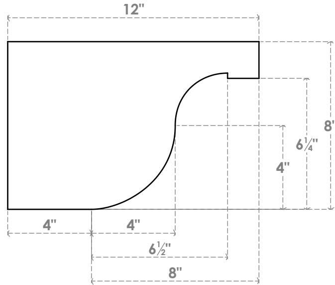
SIDE PROFILE
